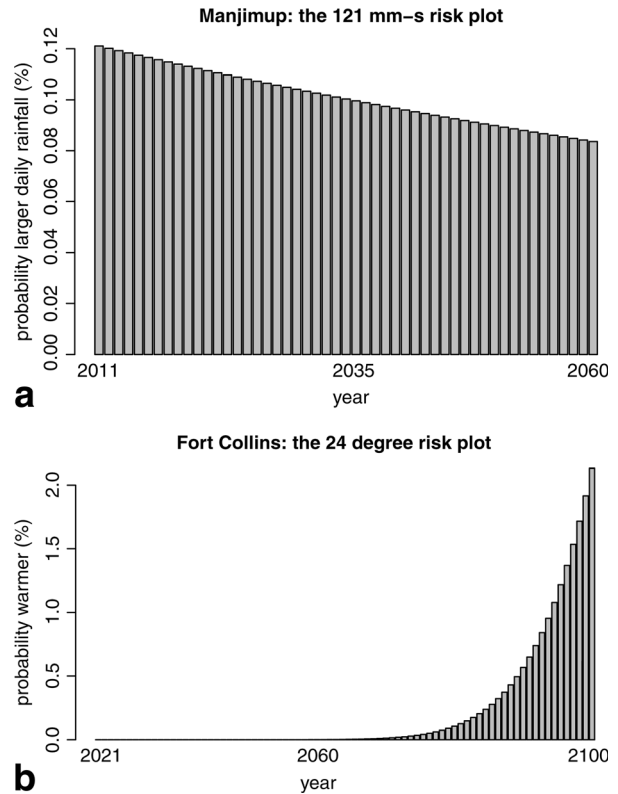
Figure 3. Risk plots. (a) Probability that the largest daily rainfall in Manjimup is greater than 121 mm. (b) Probability that the yearly minimum temperature in Fort Collins is warmer than 24^{\circ}\text{F} .
