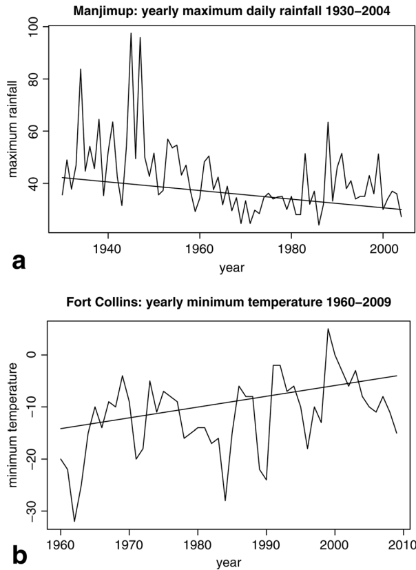
Figure 2. The data. (a) Largest daily rainfall (mm) during winter by year in Manjimup. Line is estimated location parameter (= 37% quantile) in fitted GEV distribution. (b) Lowest daily minimum temperature ( ^{\circ}\text{F} ) by year in Fort Collins. Line is estimated location parameter (= 63% quantile) in fitted GEV distribution for minima.
