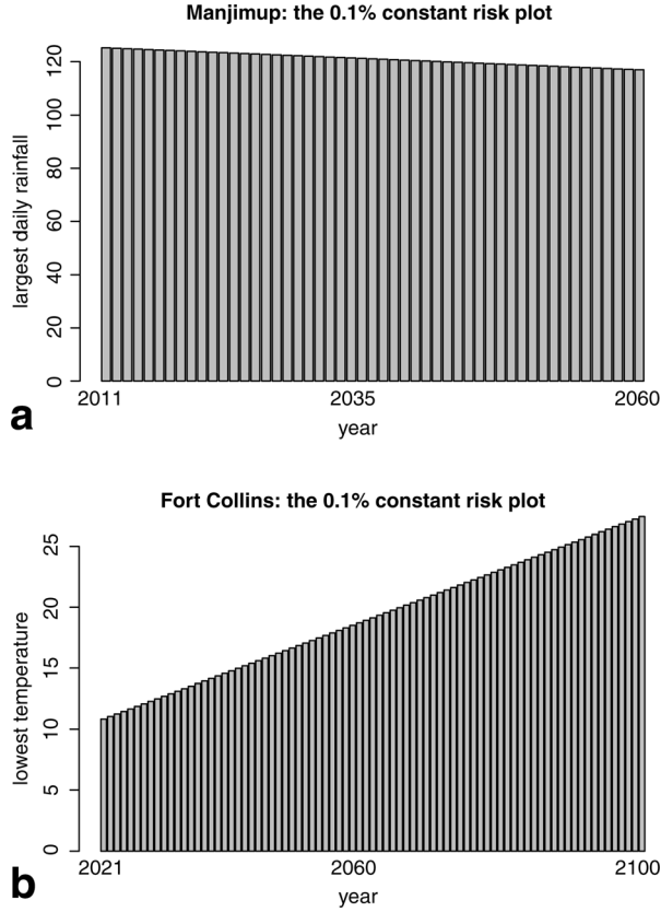
Figure 4. Constant risk plots. (a) The probability that the largest daily rainfall in a year in Manjimup is greater than the value shown for this year in plot is 0.1%. (b) The probability that the minimum temperature in a year in Fort Collins is higher than the value shown for this year in plot is 0.1%.
